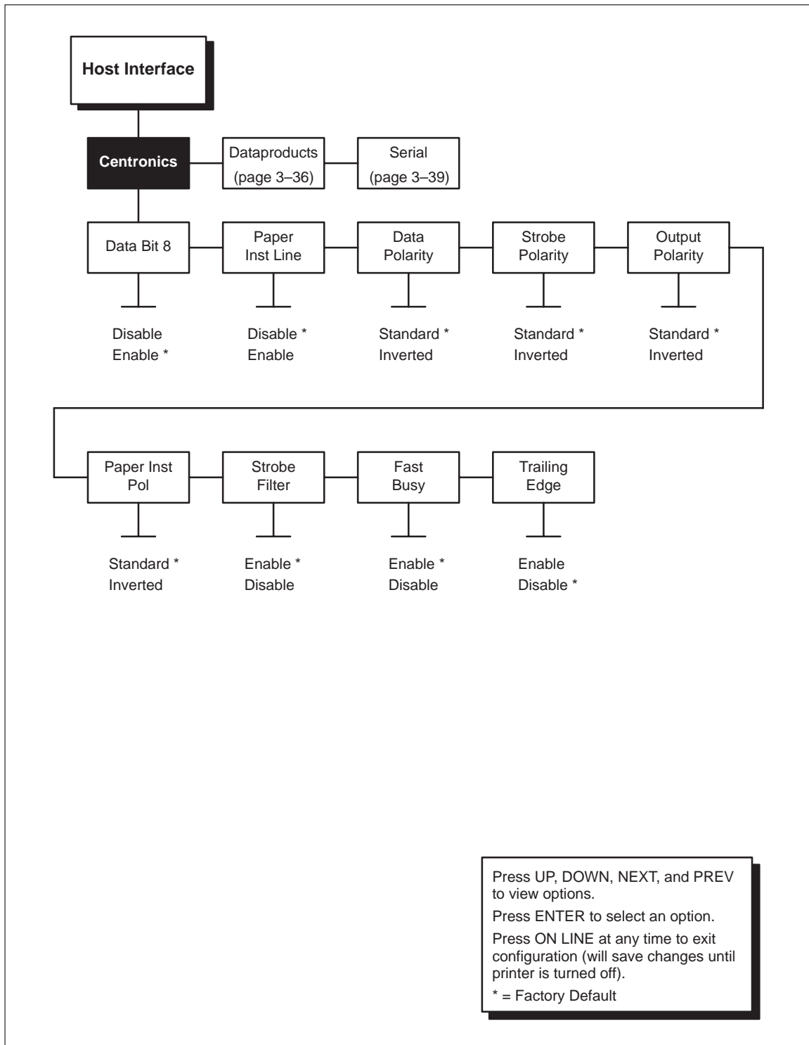
Figure 3-9. Centronics Interface Menu
