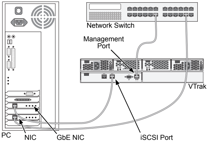
Figure 15. VTrak DAS connections
