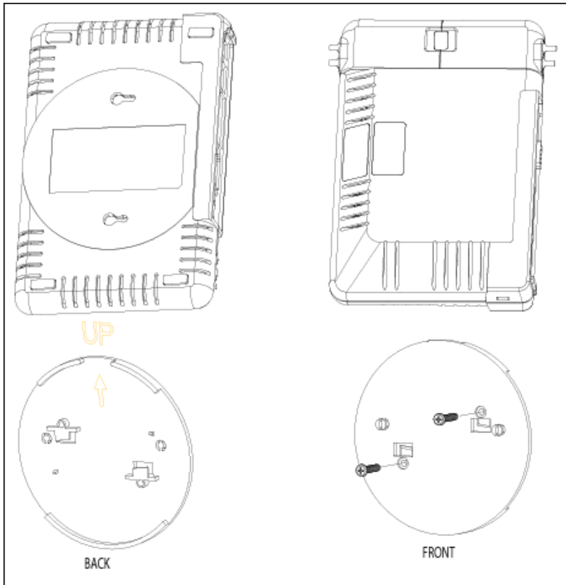
Figure 2-5 AP-700 Mounting Plate
