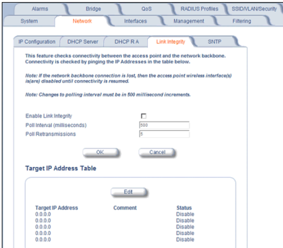
Figure 4-7 Link Integrity Configuration Screen
