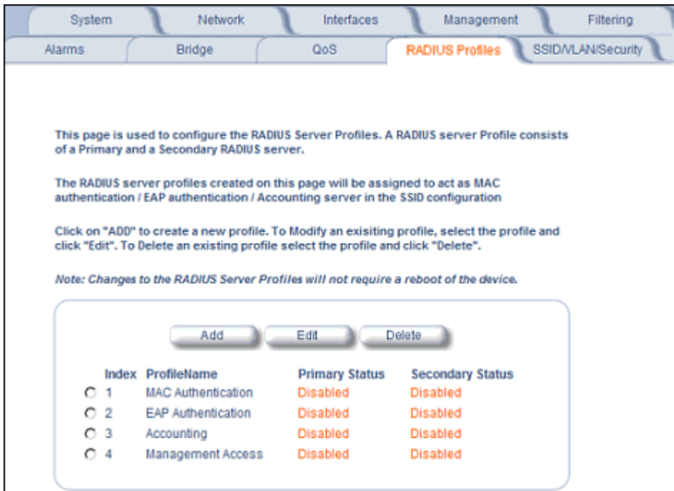
Figure 4-34 RADIUS Server Profiles
