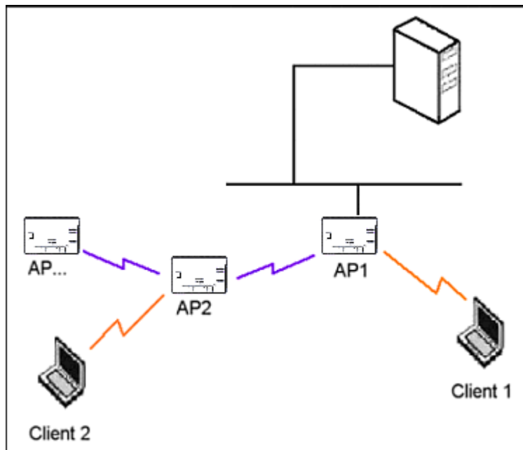
Figure 4-13 WDS Example
