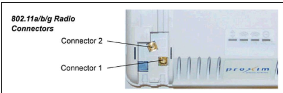
Figure 2-2 AP-700 Antenna Connectors
