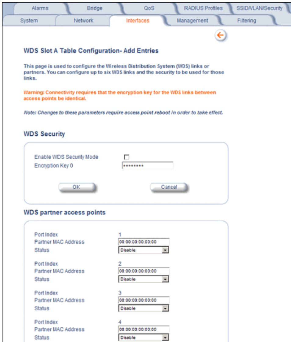
Figure 4-15 Adding WDS Links
