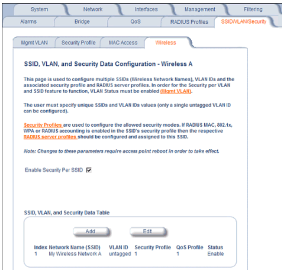
Figure 4-44 SSID/VLAN Configuration (VLAN Tagging Enabled)
