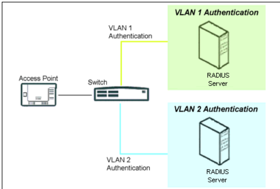
Figure 4-33 RADIUS Servers per VLAN
