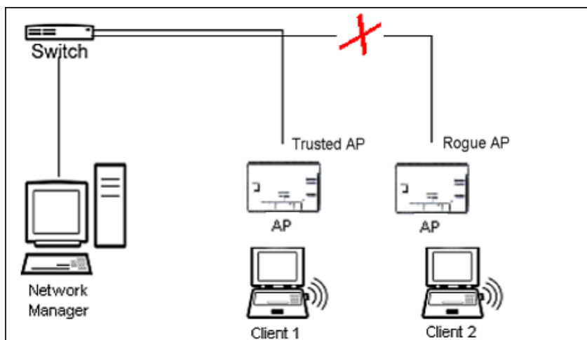
Figure 4-25 Preventing Rogue AP Attacks
