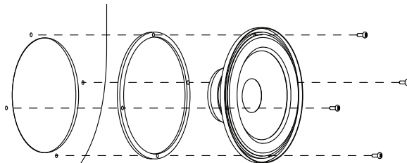
Figure 1 Mounting the speaker in a factory location.
