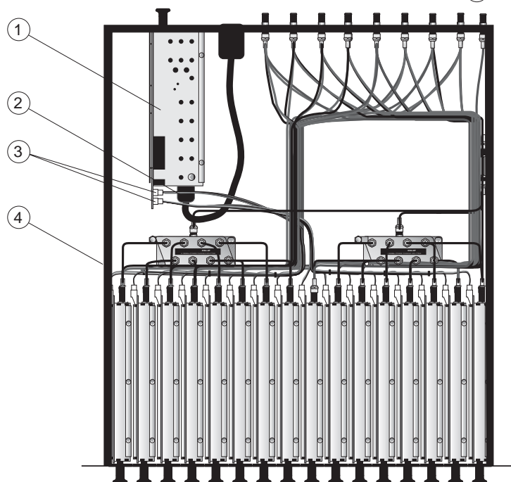
MPC-16 Top View
