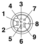
CN-1 (DIN 9-pin side)
