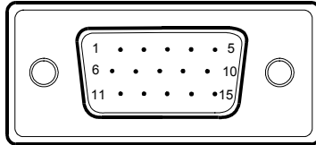
15 - Pin Color Display Signal Cable
