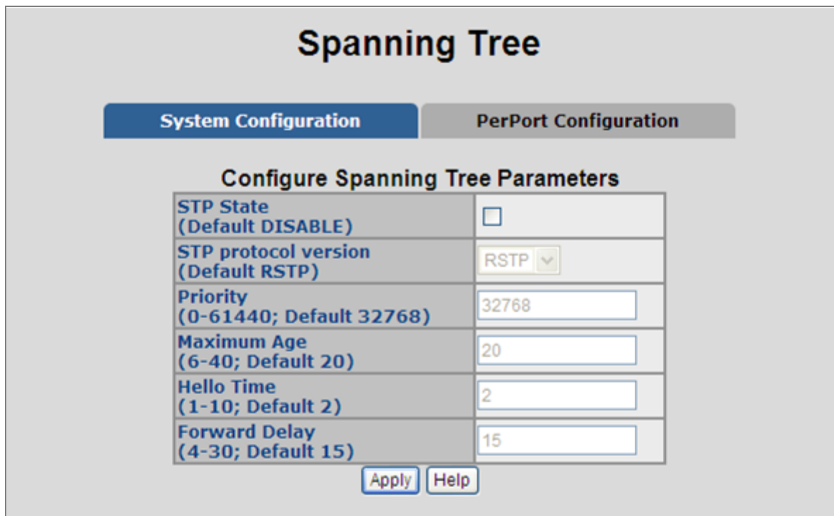
Figure 4-5-4: RSTP System Configuration interface
