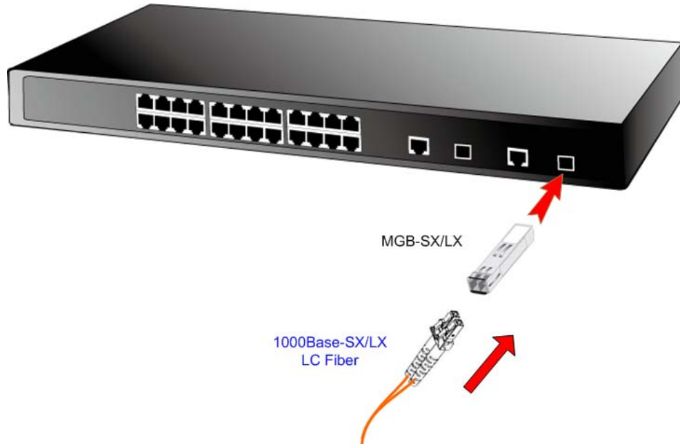
Figure 2-10: Plug-in the SFP transceiver
