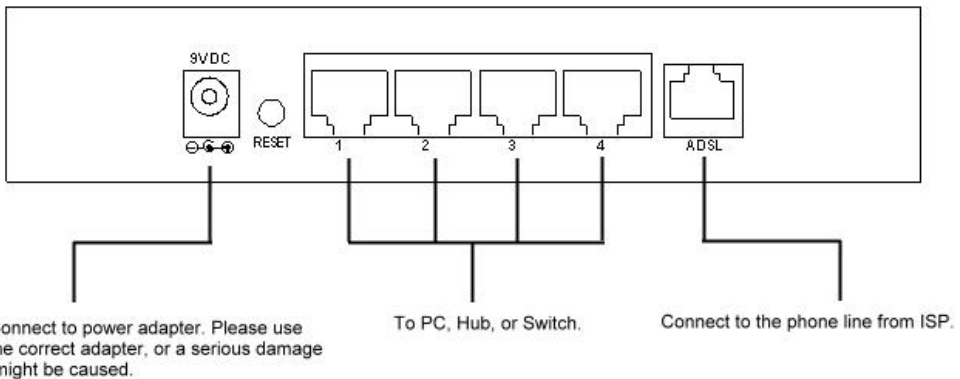
Figure 2-1: Installation Diagram
