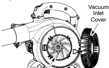
Vacuum Inlet
