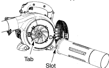
Vacuum Inlet
