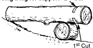
Using a log for support
