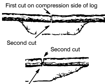
First cut on compression side of log
