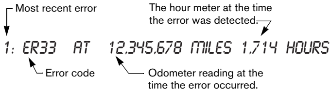
Diagram 10: Error log
