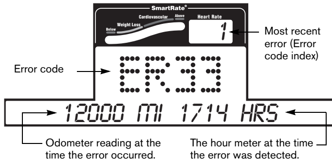
Diagram 7: Error log
