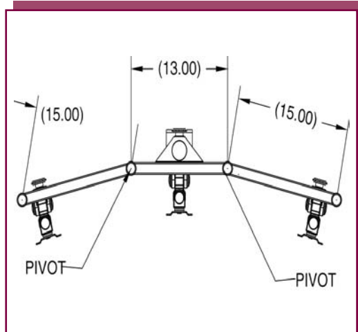
Top View (Measurements in Inches)
