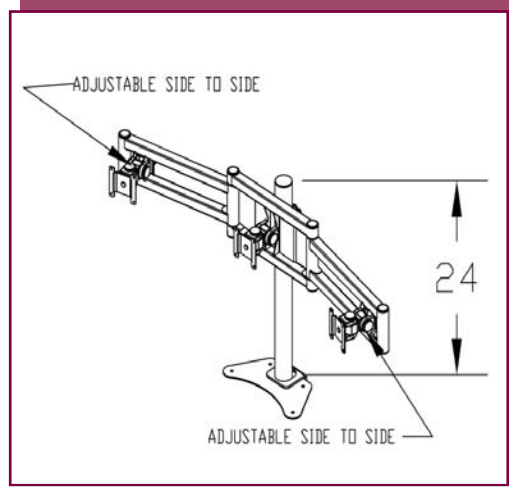
PMPI Multi-Monitor Series (Measurements in Inches)
