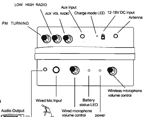
PWMA200 Single channel main frame (With Built-in Rechargeable battery)
