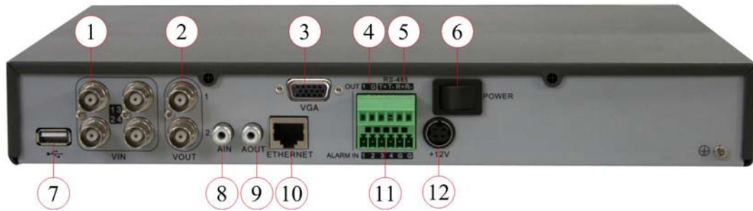
Fig 2-1 QSC26404 Rear Panel
