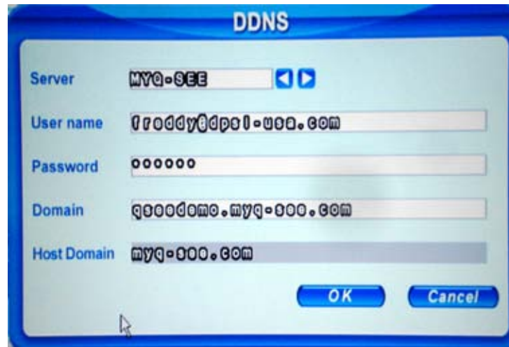
Image 4.14 Configuration DDNS
