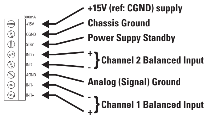
Figure 2. Eight screw clamp terminals offer connections for inputs, remote on/off control, and a 15-volt DC supply.
