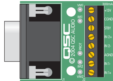
Figure 1. The DDI-11 and its control/monitoring connections.
