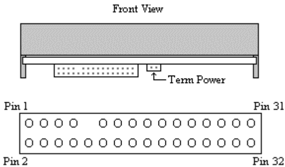
Front Option Connector - J3
