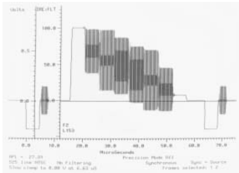
1 Horizontal Period of TVBar_75Image as it would appear on a TV waveform analyzer connected to the 801GX's TV output
