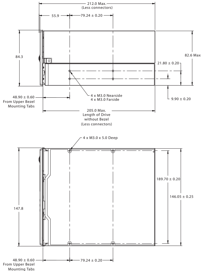
Figure 4 Internal LTO-3 Tape Drive Mounting Dimensions
