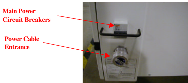
Figure 1.3 Circuit Breaker / Power Cable Entrance
