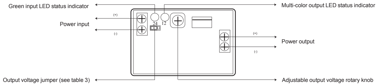
Figure 1 - Wiring diagram
