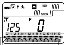
EV scale Aperture scale Clipping and Dynamic range icons Value display scale
