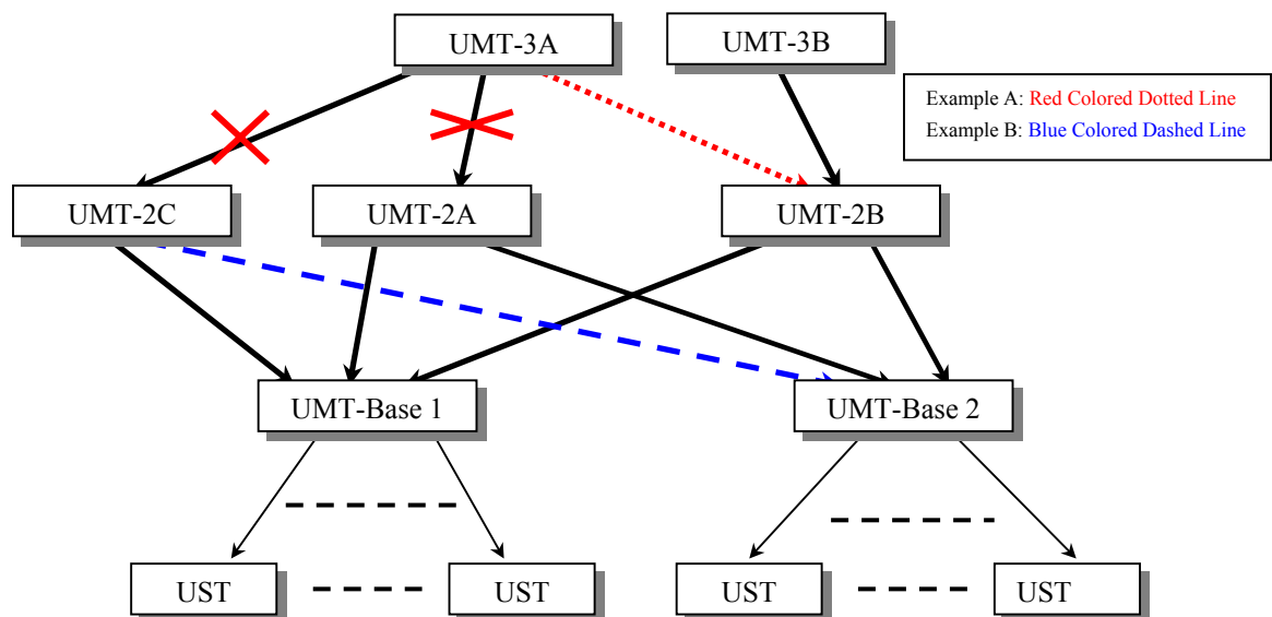
Figure 45 Multiple Base Configuration
