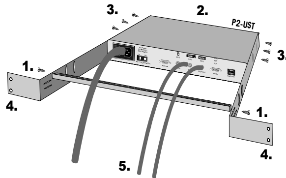
Figure 63 Rear rackmount of a P2 User Station
