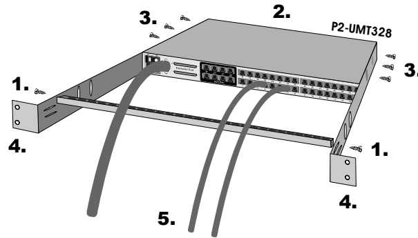
Figure 62 Rear rackmount of a P2 Base Unit
