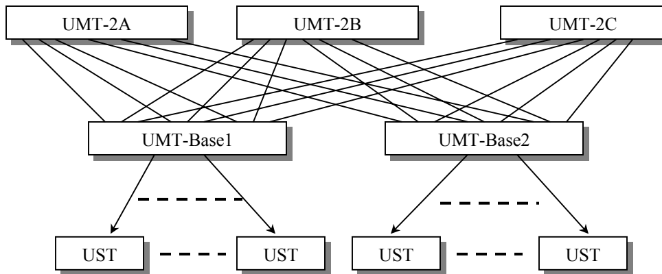
Figure 57 Recommended Redundant Configuration connection scheme
