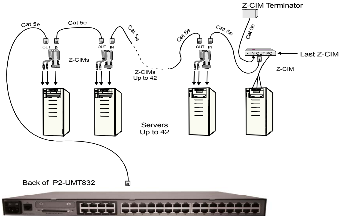
Figure 42 Connecting a Z-CIM as a Tier to Paragon II
