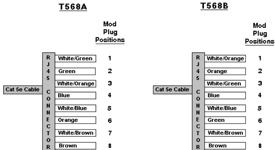
Figure 59 Cat5 Cable Diagram
