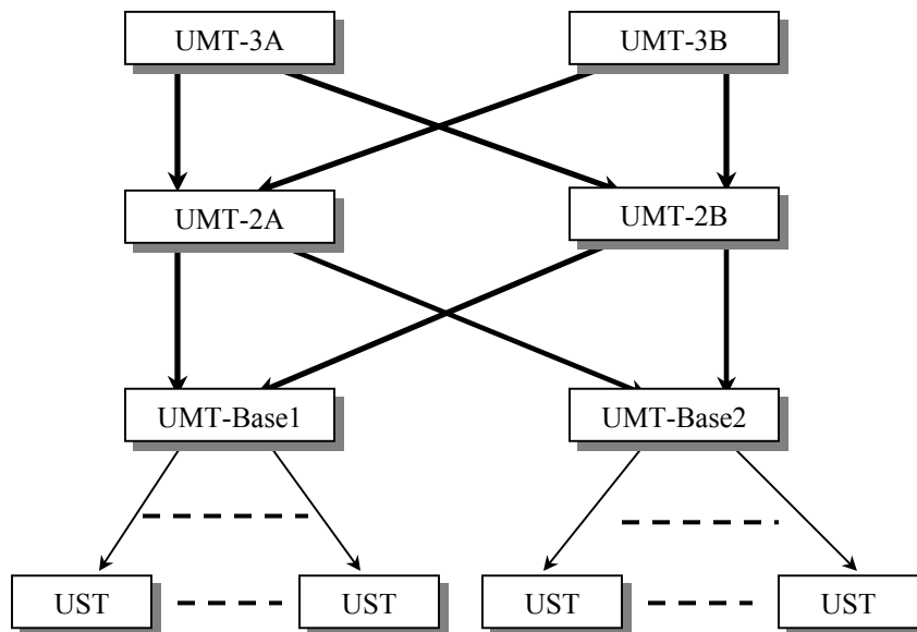
Figure 56 Redundant Configuration
