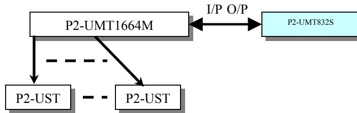
Figure 50 Stacking - Single Base Configuration with P2-UMT1664M and P2-UMT832S
