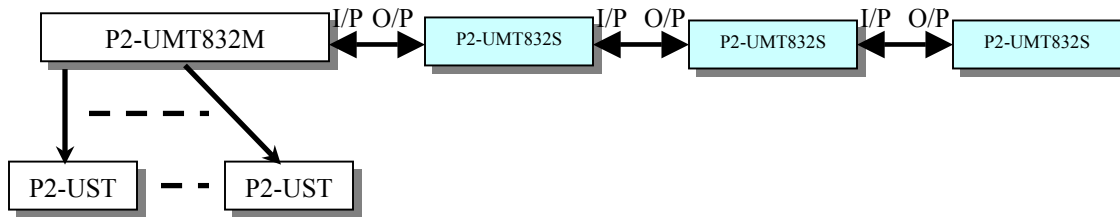
Figure 47 Stacking - Single Base Configuration with P2-UMT832M and P2-UMT832S
