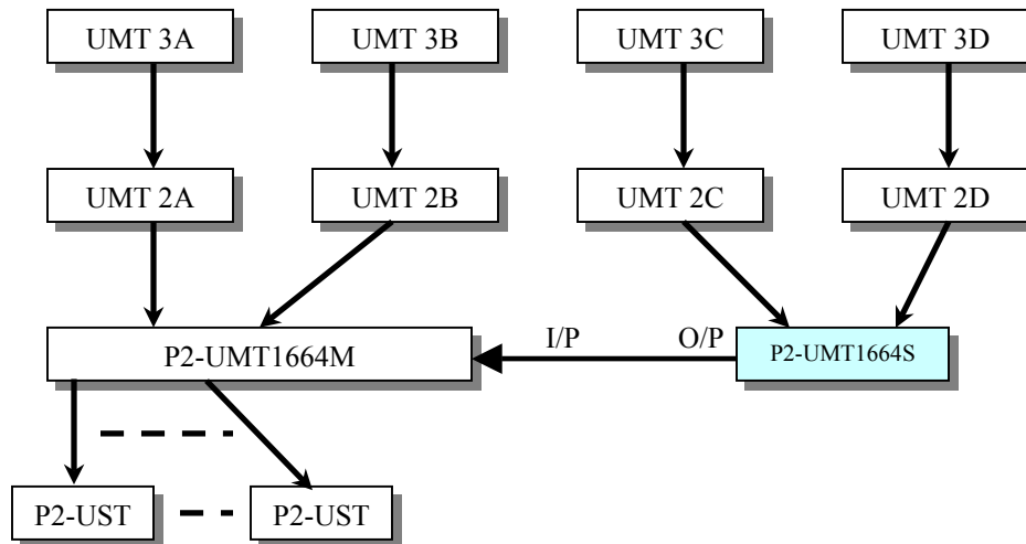
Figure 48 Stacking - Single Base Configuration with P2-UMT832M and P2-UMT832S
