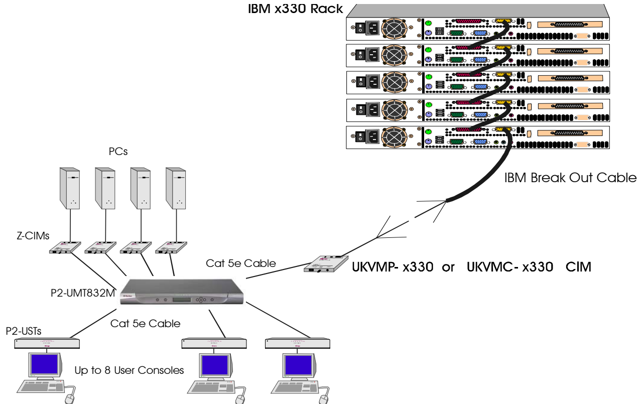
Figure 43 IBM x330 Tiered from a Paragon II Matrix Switch
