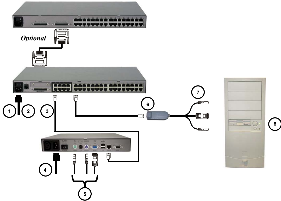
Figure 3 Installation Diagram
