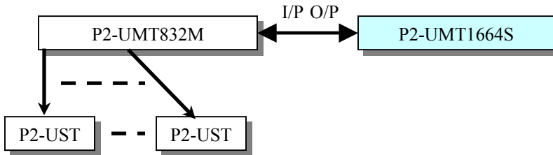
Figure 53 Stacking - Single Base Configuration with P2-UMT832M and P2-UMT1664S
