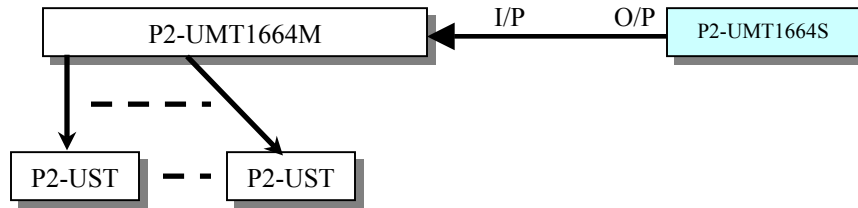
Figure 46 Stacking - Single Base Configuration with P2-UMT1664M and P2-UMT1664S
