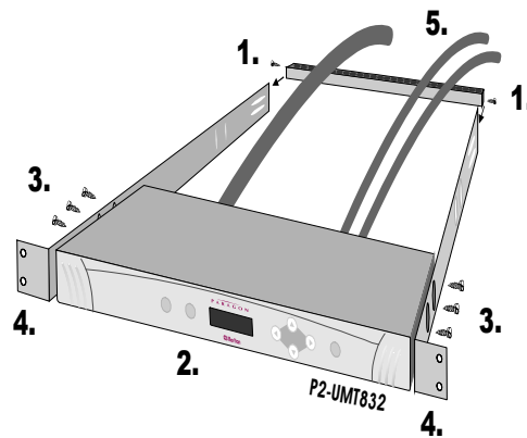
Figure 60 Front rackmount of a P2 Base Unit
