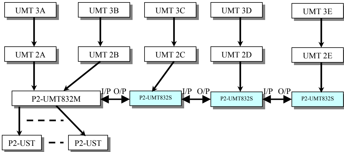
Figure 49 Stacking - Single Base Configuration with P2-UMT832M and P2-UMT832S
