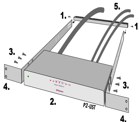
Figure 61 Front rackmount of a P2 User Station
