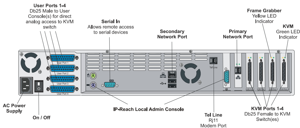
Back Panel of IP-Reach TR Series
