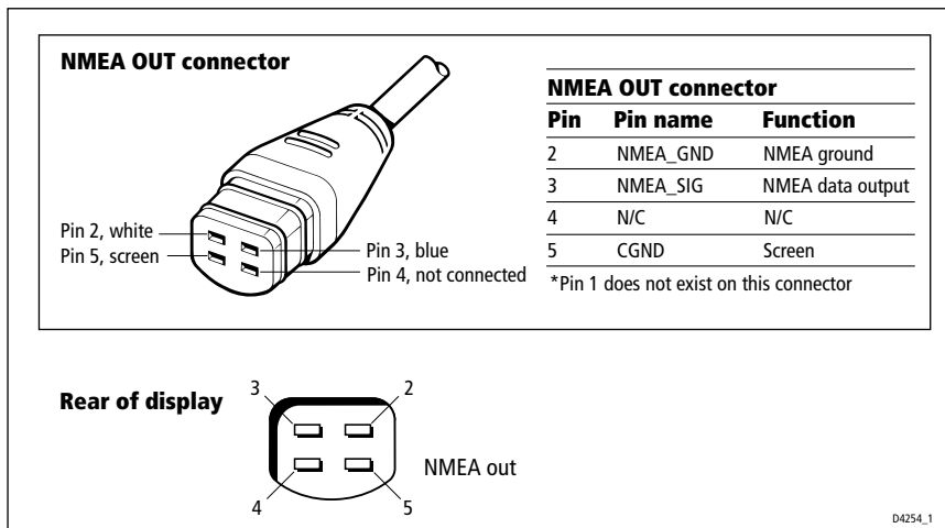
Figure 8-18: NMEA Output Connector
