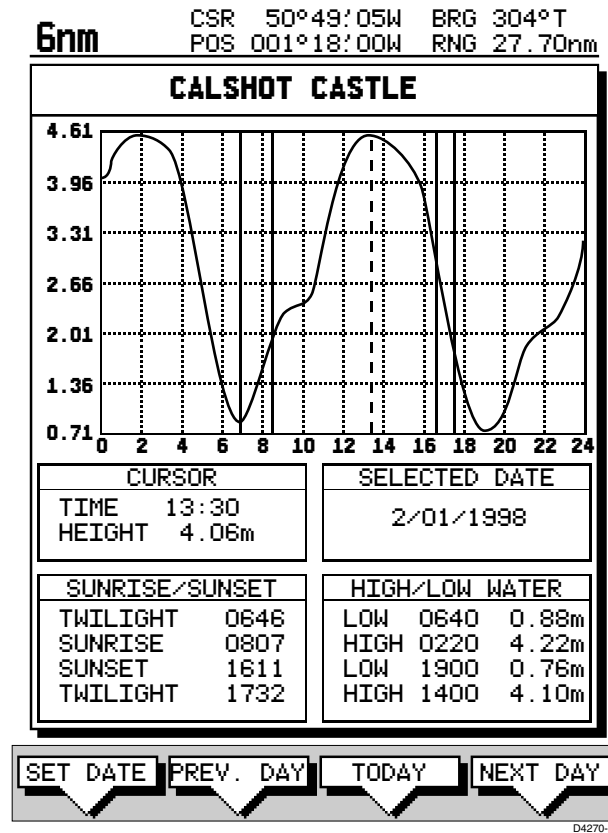
Figure 5-3: Tide Data
