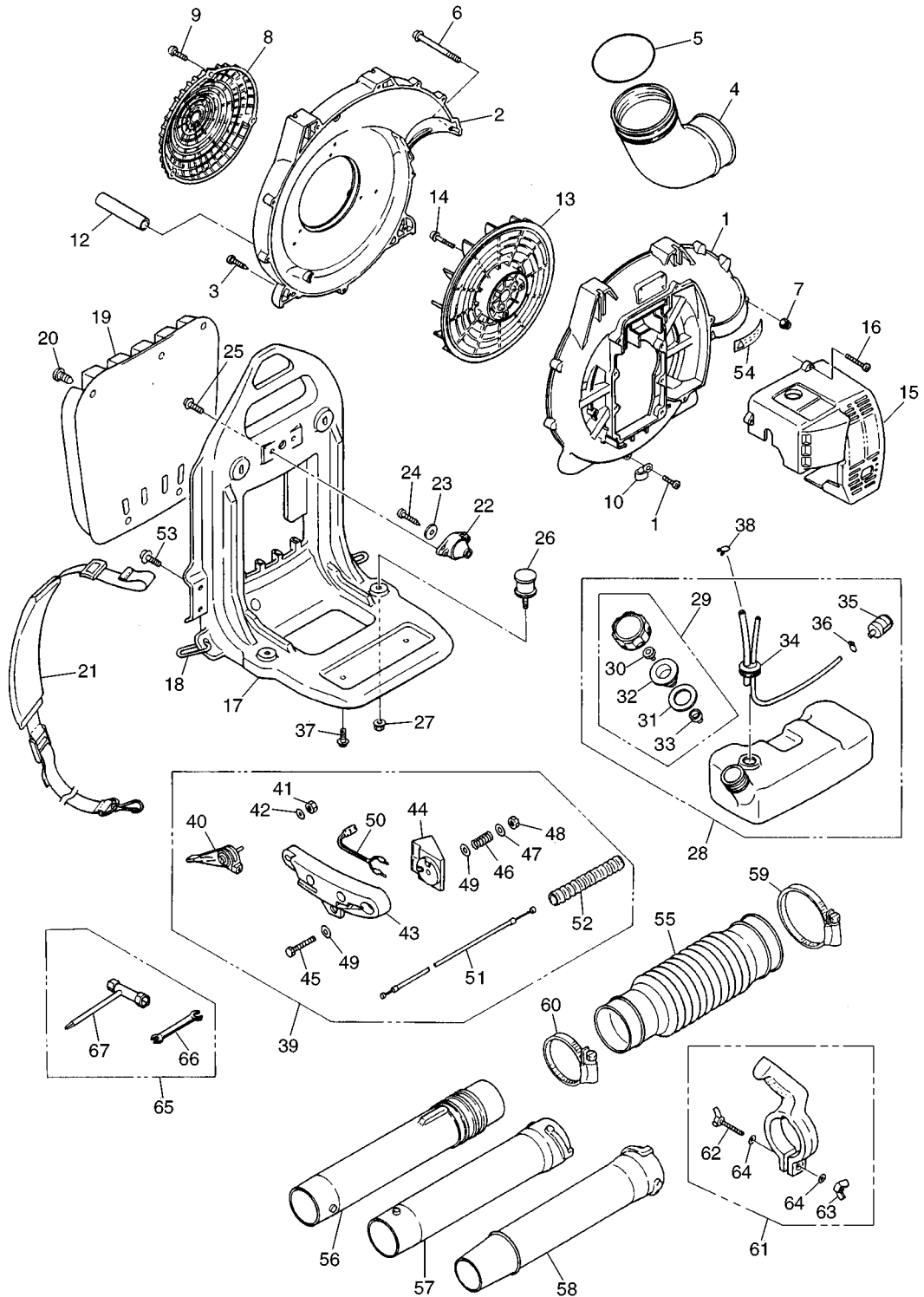
Fig.3 BLOWER GROUP
