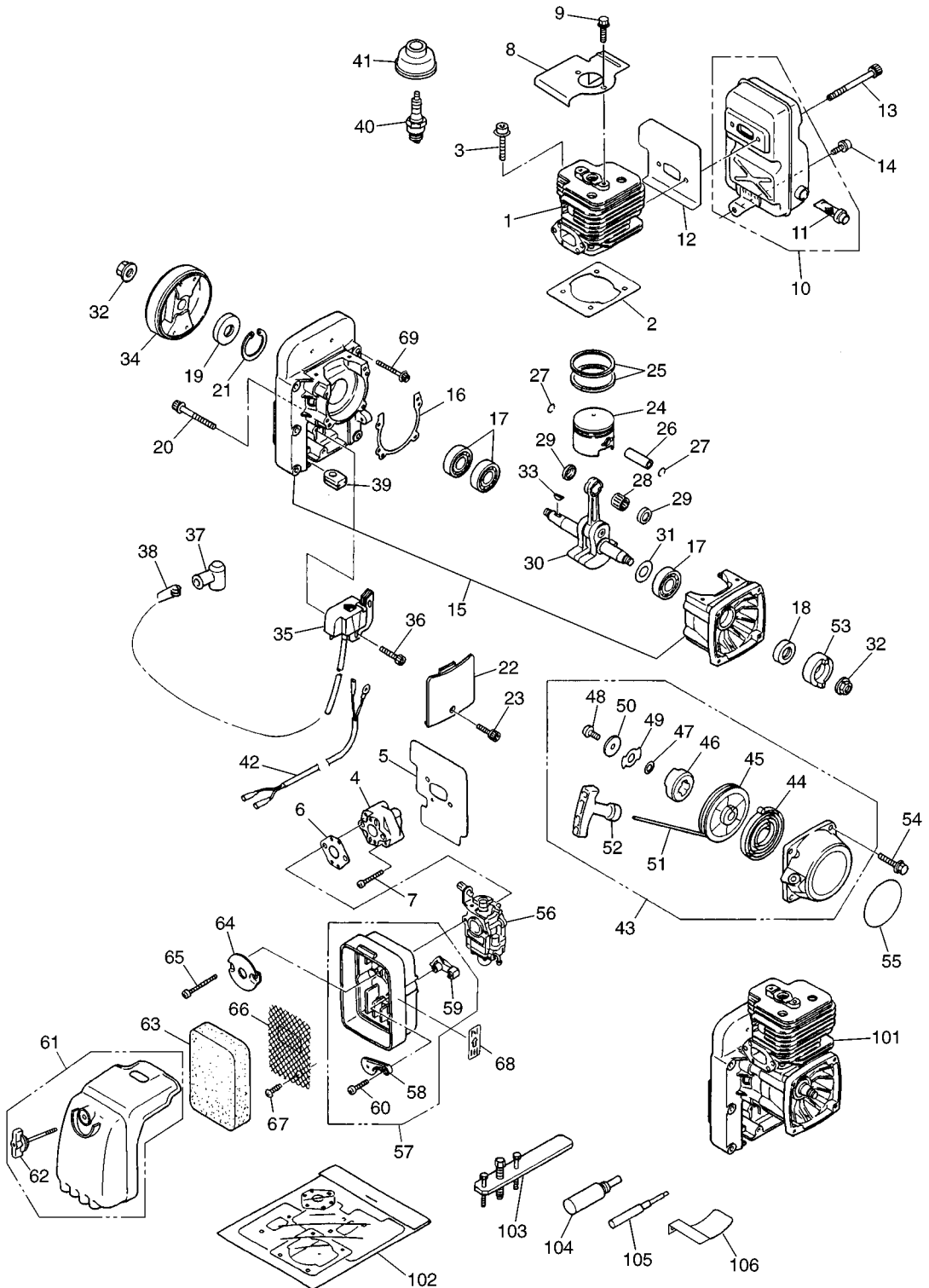
Fig.2 ENGINE GROUP
