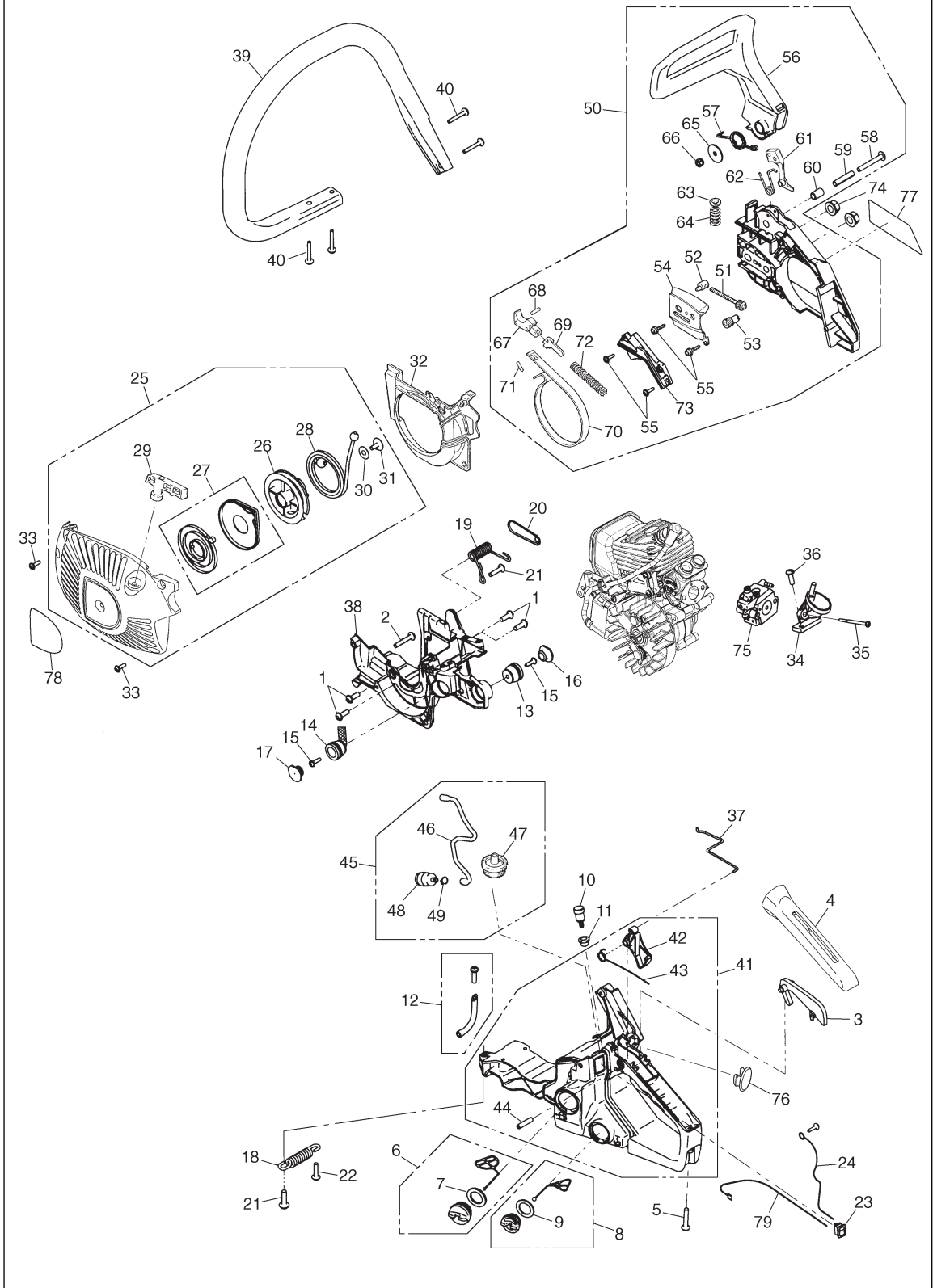
Fig.2 POWER UNIT (S/N 720401 and up)
