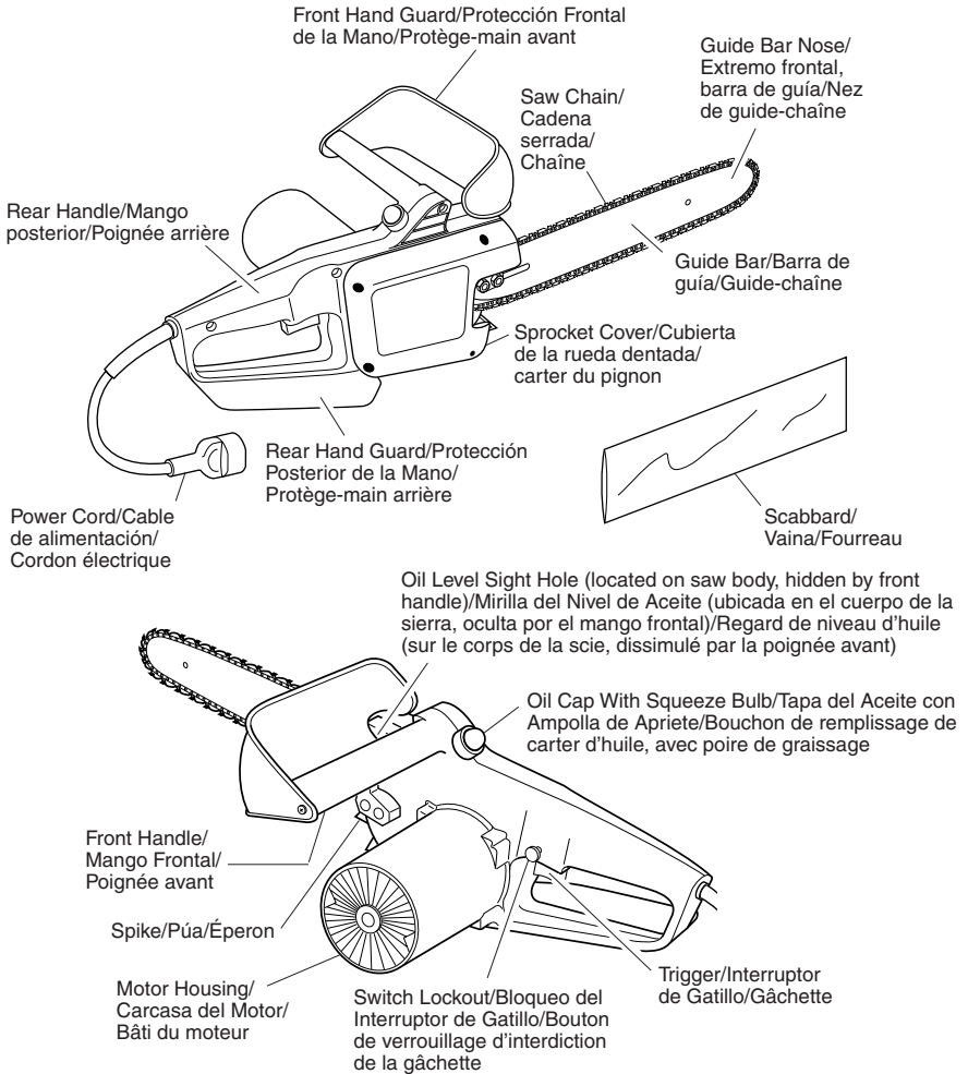
Figure 1 - Electric Chain Saw
