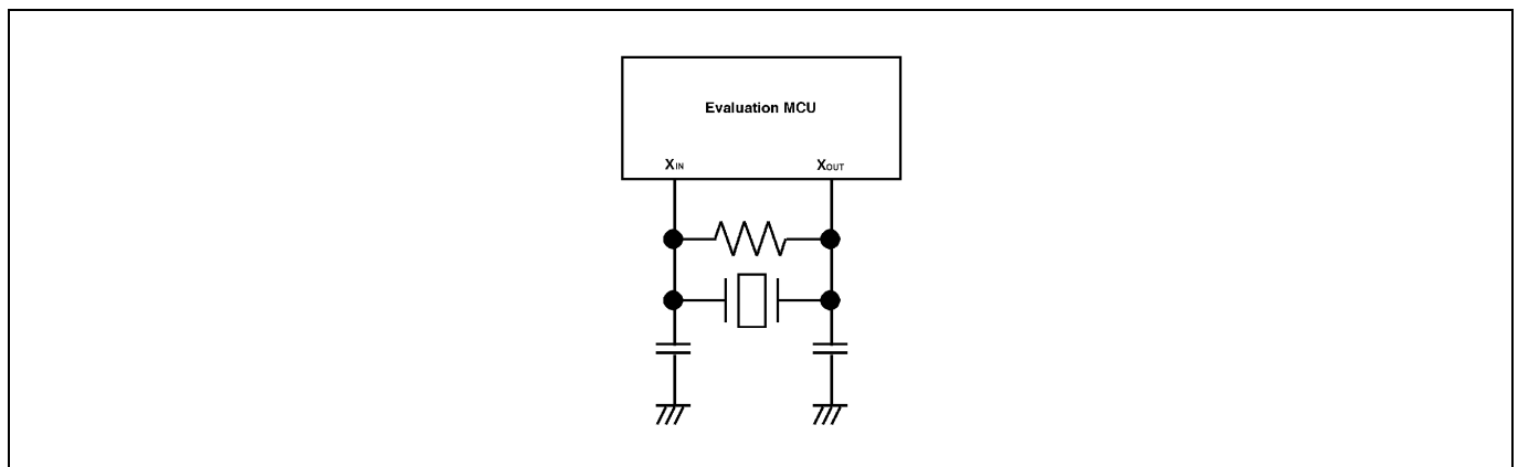
Figure 2.22 Circuit in which oscillation does not occur
