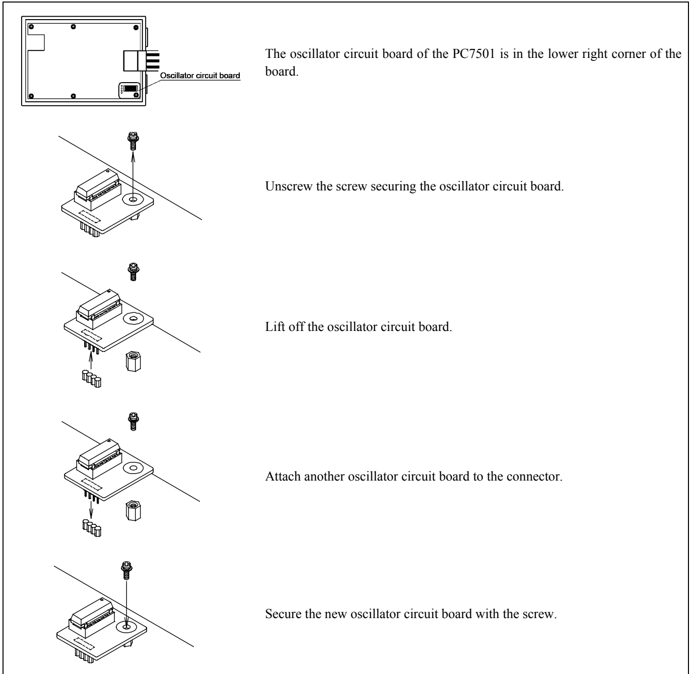
Figure 2.18 Replacing oscillator circuit boards
