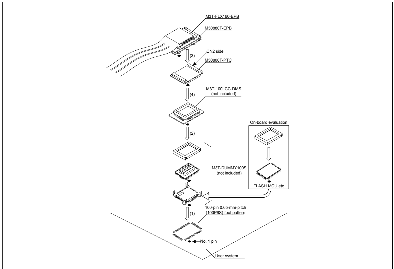
Figure 2.9 Connecting to a 100-pin 0.65-mm-pitch foot pattern (1/3)
