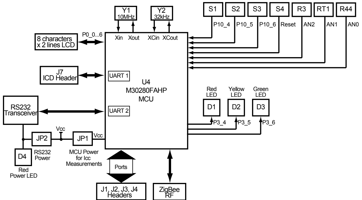
Figure 5-2: RZB-ZMD16C-ZDK Block Diagram
