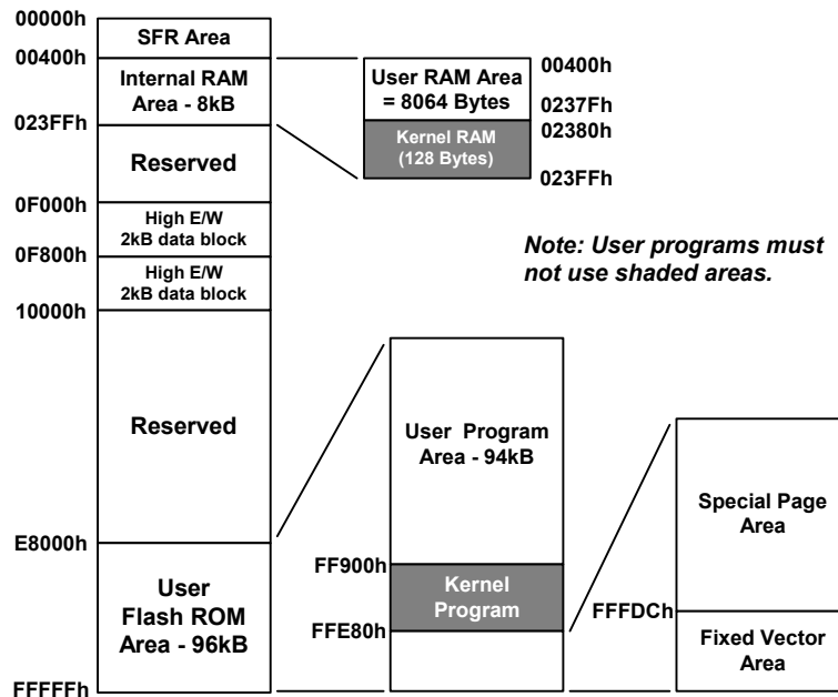
Figure 7-1: M30280FAHP Memory Map with the Kernel Program
