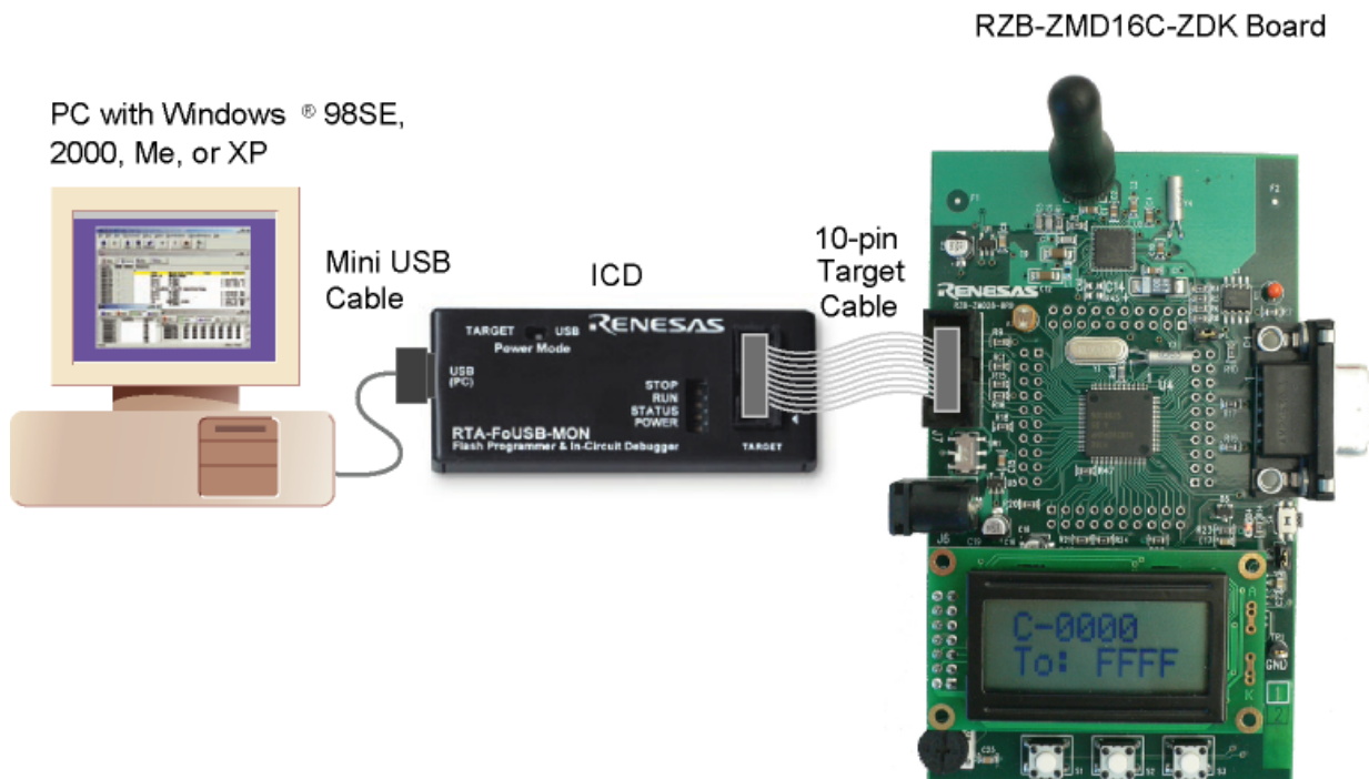
Figure 4-2 ZDK Development System Connectivity
