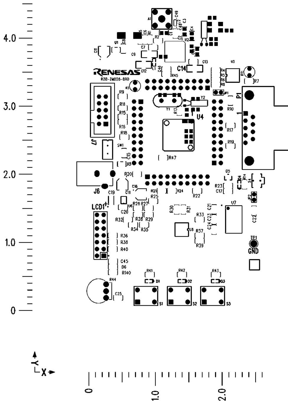
Figure E-1: PCB Top View
