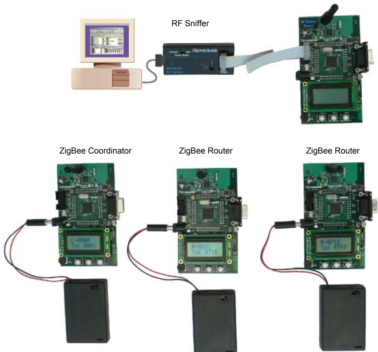
Figure 4.1: ZigBee Demo Kit Setup
