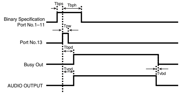
Timing Chart (PLAY)
