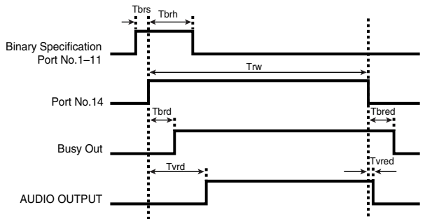
Timing Chart (Rec)
