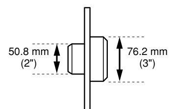
Media flange
