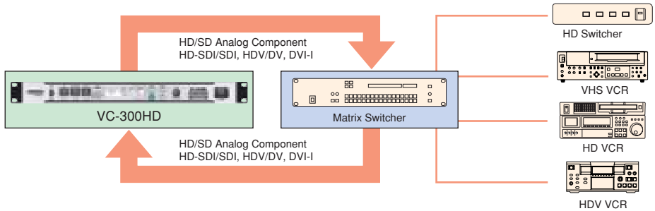
Figure 2. A multi-format converter is indispensable during post production, when many and varied video formats have to be dealt with. Used together with a matrix switcher, the VC-300HD can greatly boost efficiency and simplify conversion tasks from basic conversion to aspect ratio control, color adjustment, and other tweaks.
