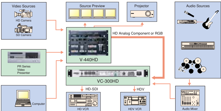
Figure 3. Production of live performance and studio video shot using various sources can be carried out using video mixing systems such as the Edirol V-440HD multi-format video mixer. If a VC-300HD is included in the system, the video line and audio can be combined during acquisition. Audio delay control, built into the VC-300HD, enables audio to be synchronized with the video.
