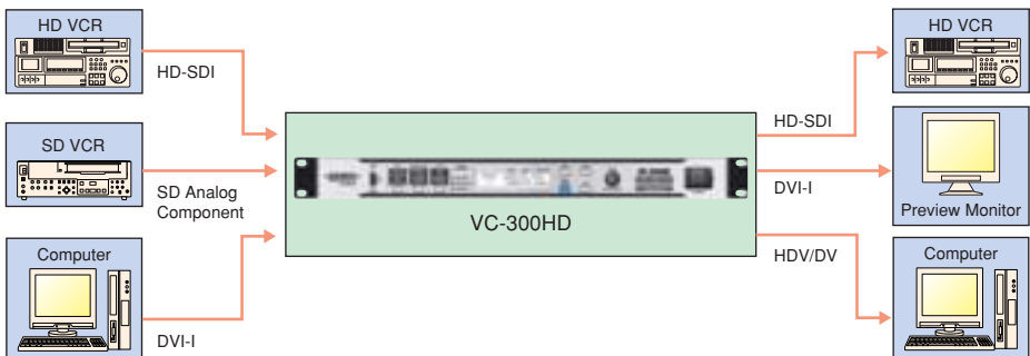
Figure 1. Using the VC-300HD various video formats can be acquired as HDV or DV.
