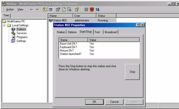
Figure 11. Start/Stop window
