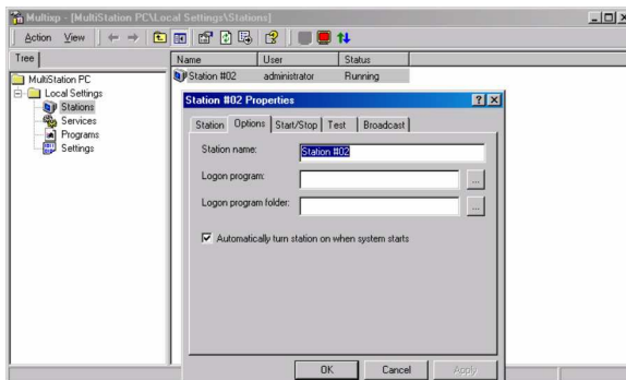
Figure 10. Station options
