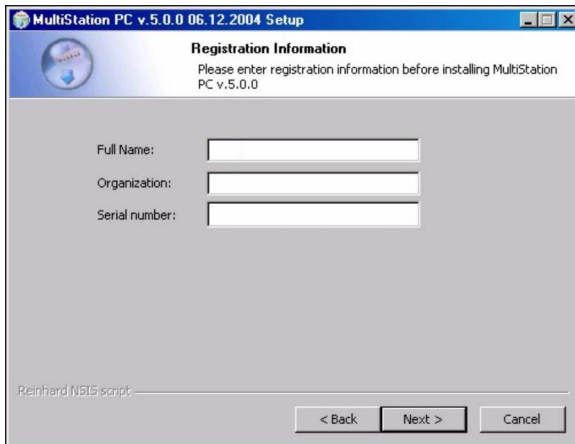
Figure 5. User information
