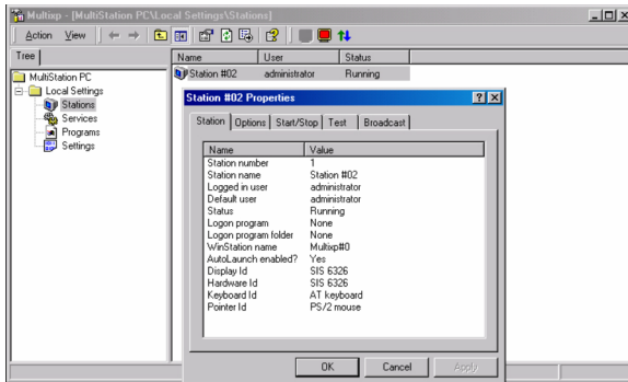
Figure 9. Station Properties
