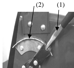
Figure 2. Height adjustment
