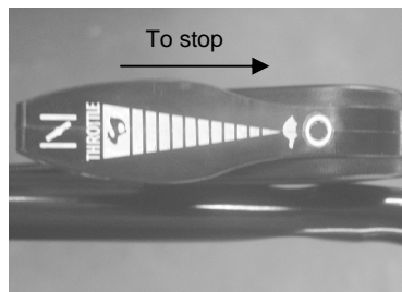
Figure 8. Throttle Control - ("CHOKE" | / | Position)
