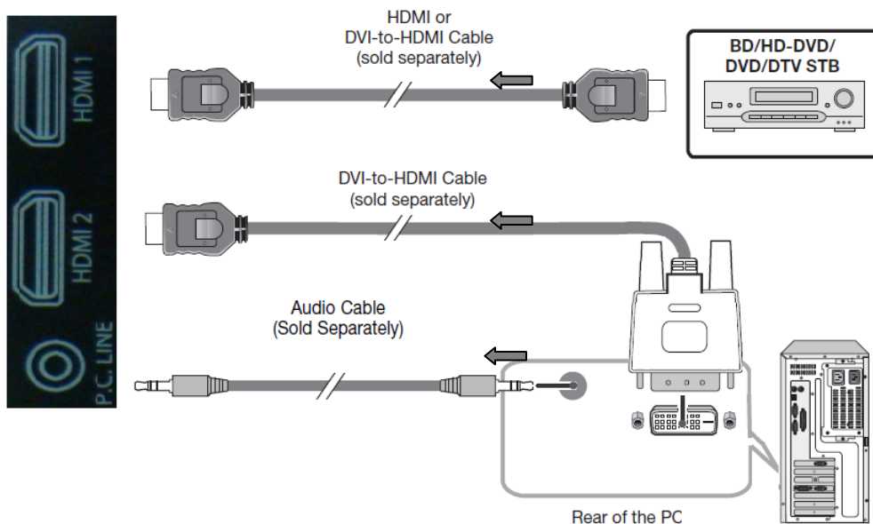
Figure 3-1. HDMI Connections
