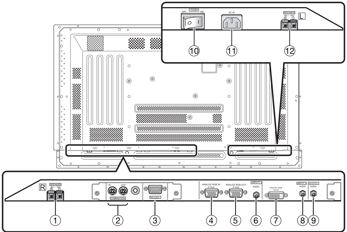
Figure 2-2. PlasmaWall Connectors
