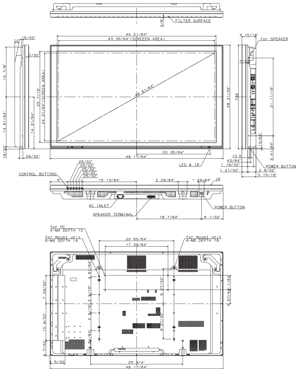
Figure 7-1. PlasmaWall Model PL-50XA Dimensions
