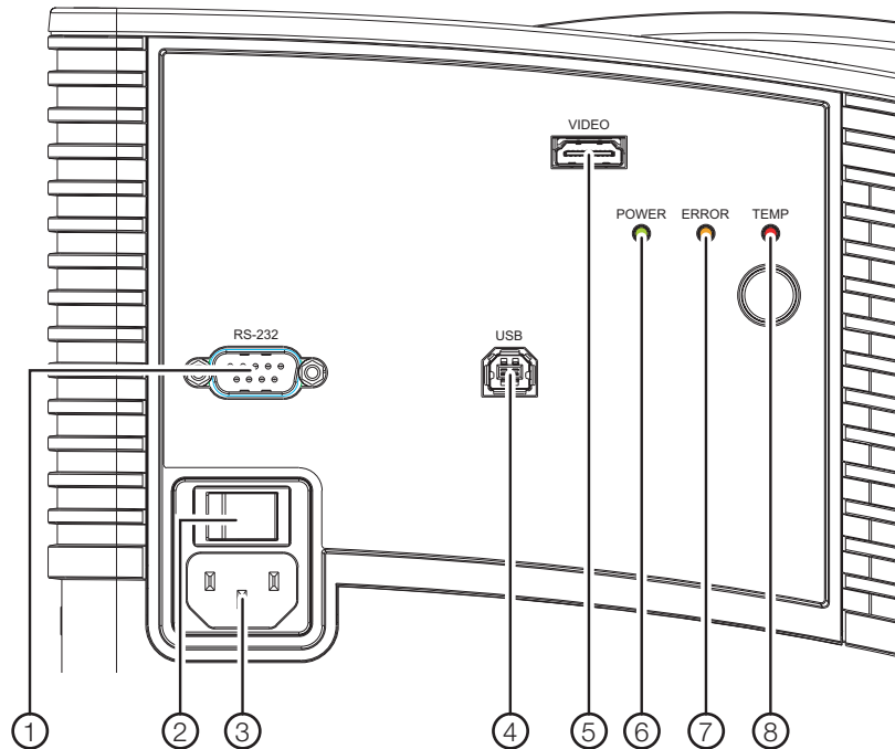
Figure 2-2. LS-100d Input Panel
