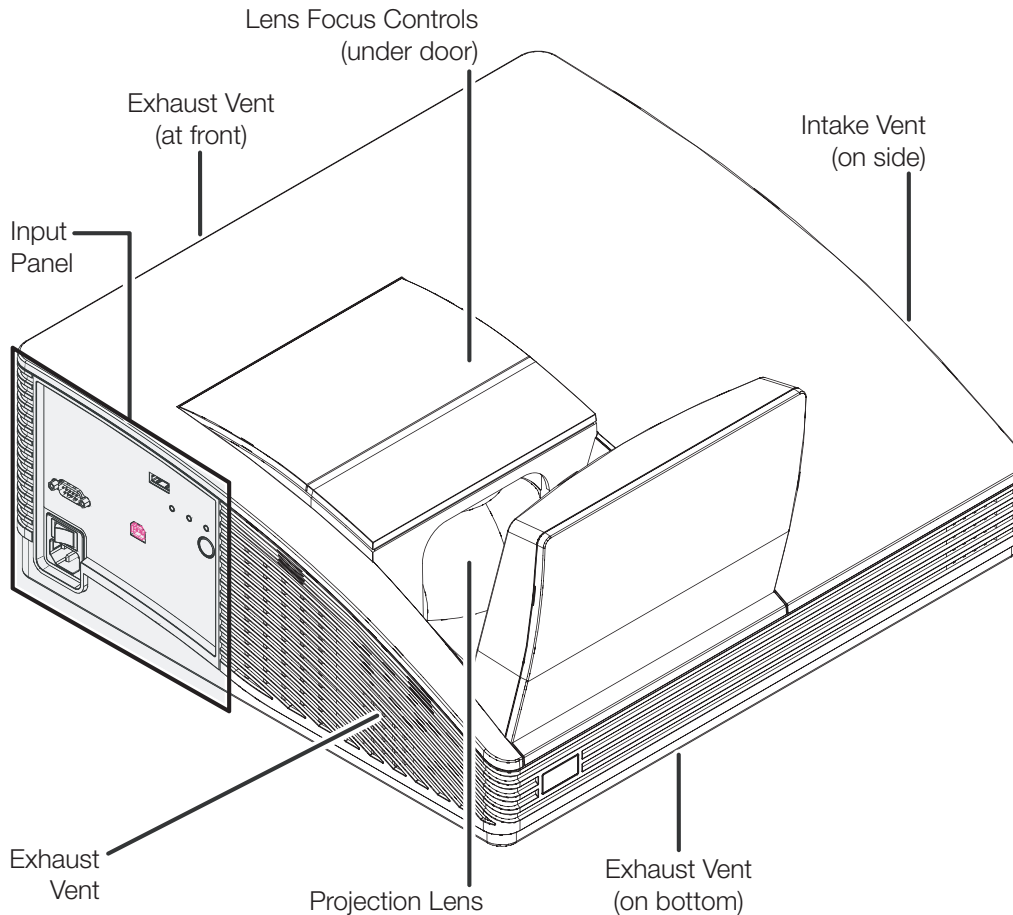
Figure 2-1. LS-100d Rear/Side/Top View
