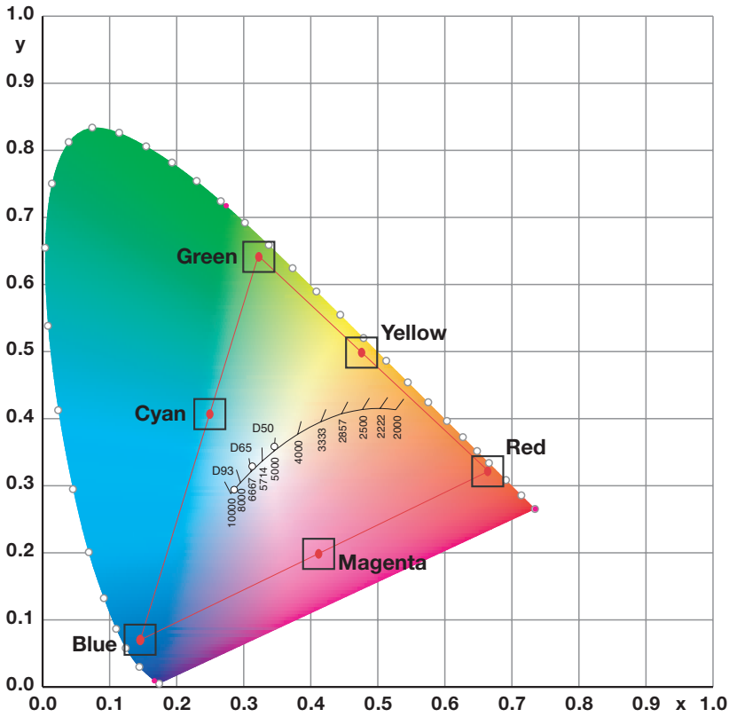
Figure 4-7. CIE 1931 Chromaticity Diagram
