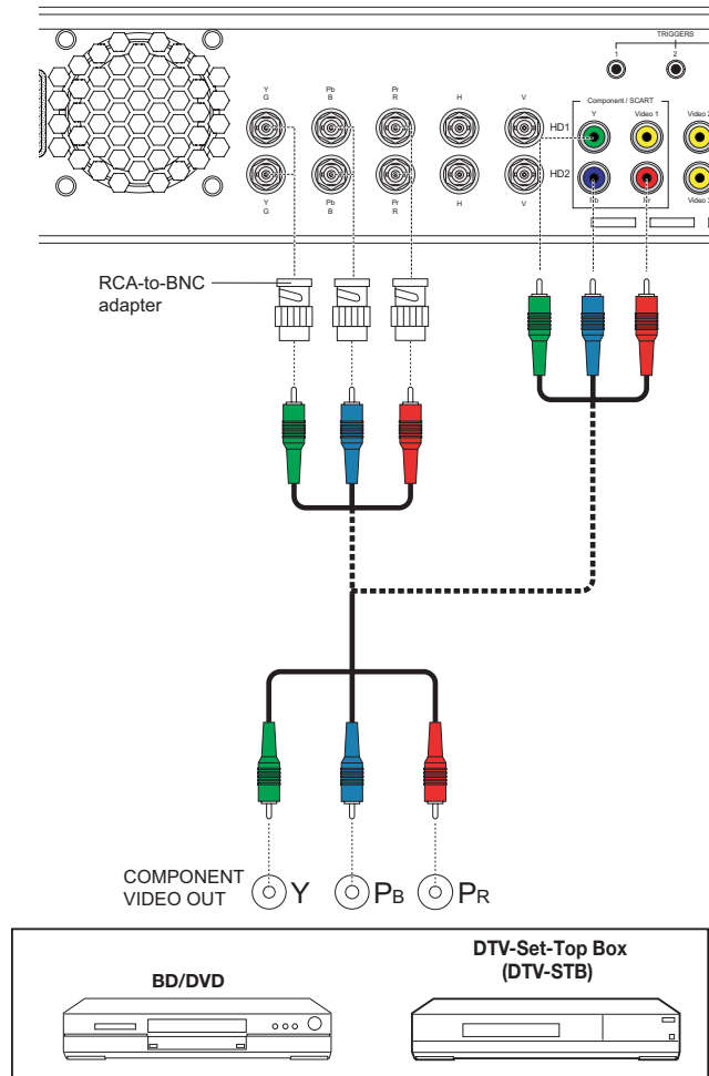
Figure 3-12. Component Video Source Connections
