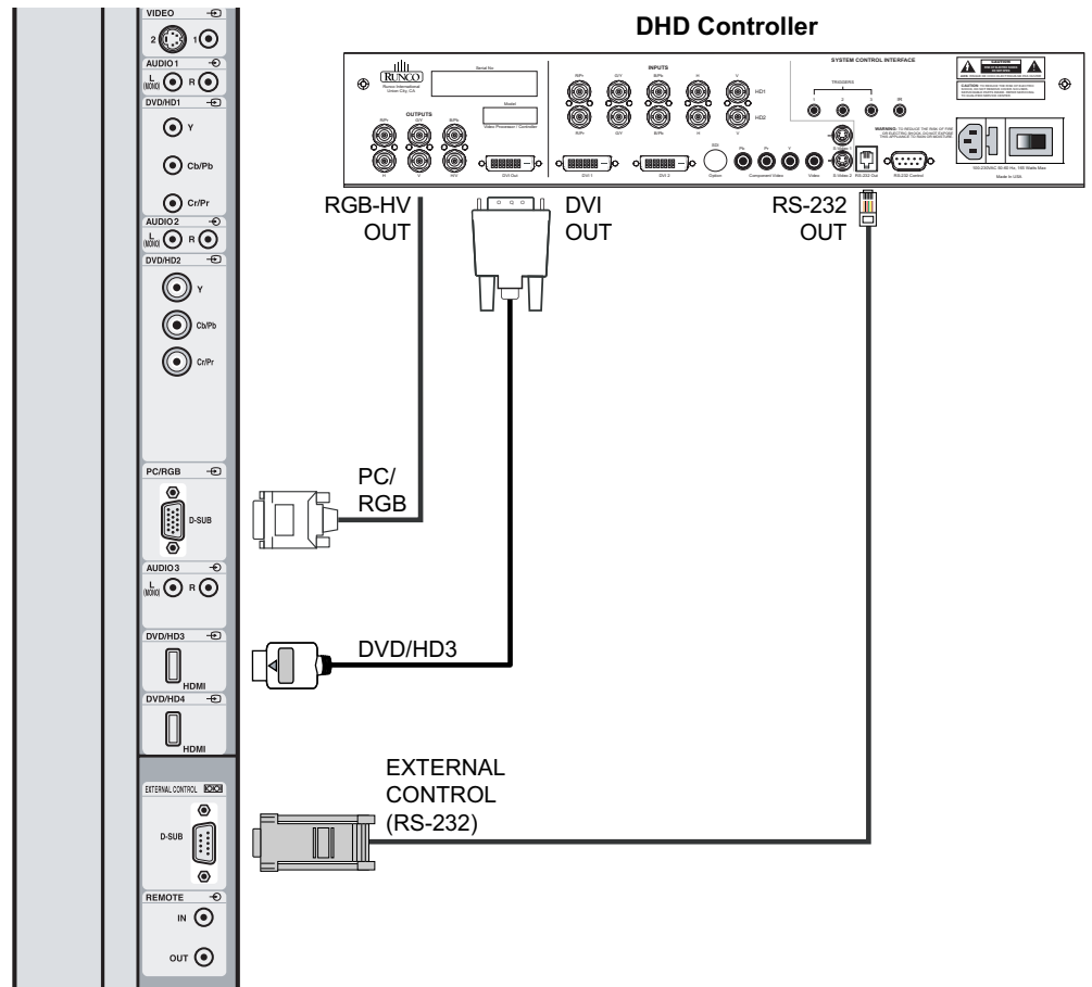
Figure 3-3. Connecting the PlasmaWall to the DHD Controller
