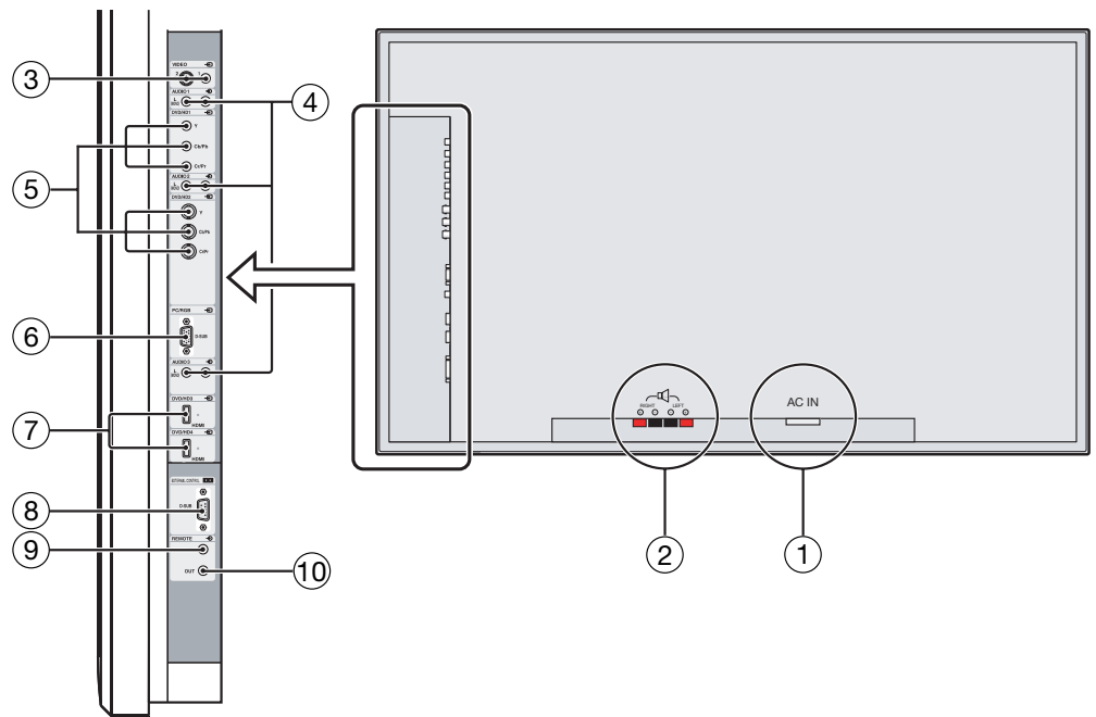
Figure 2-2. PlasmaWall Connectors
