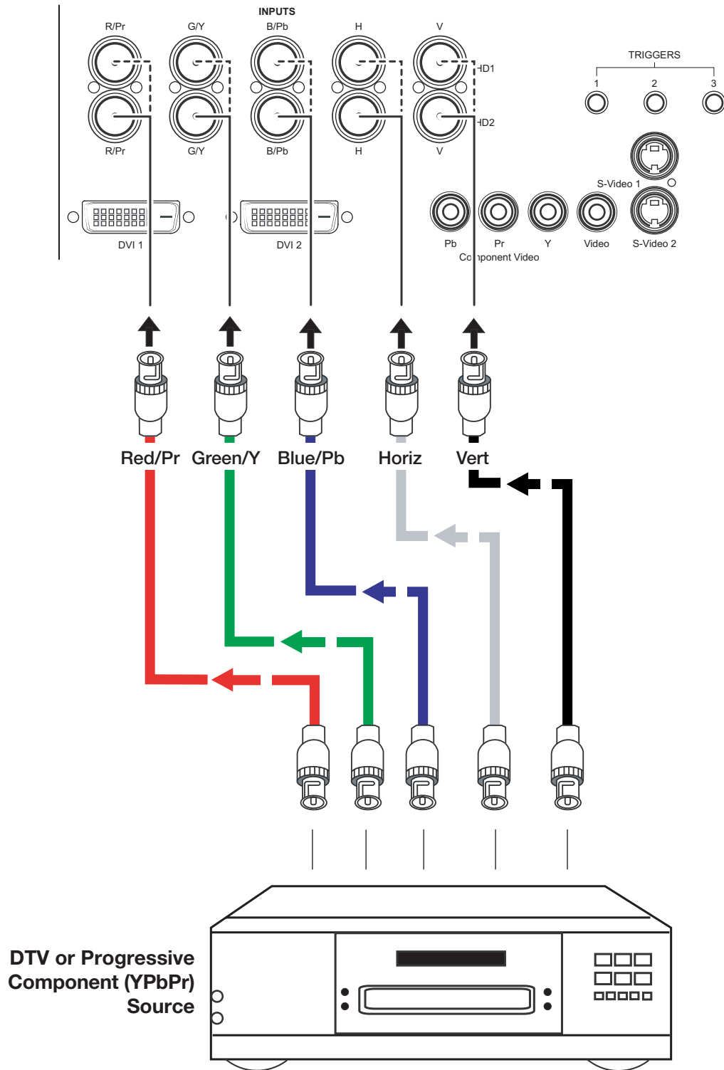
Figure 3-6. Digital (DTV) RGB Connections
