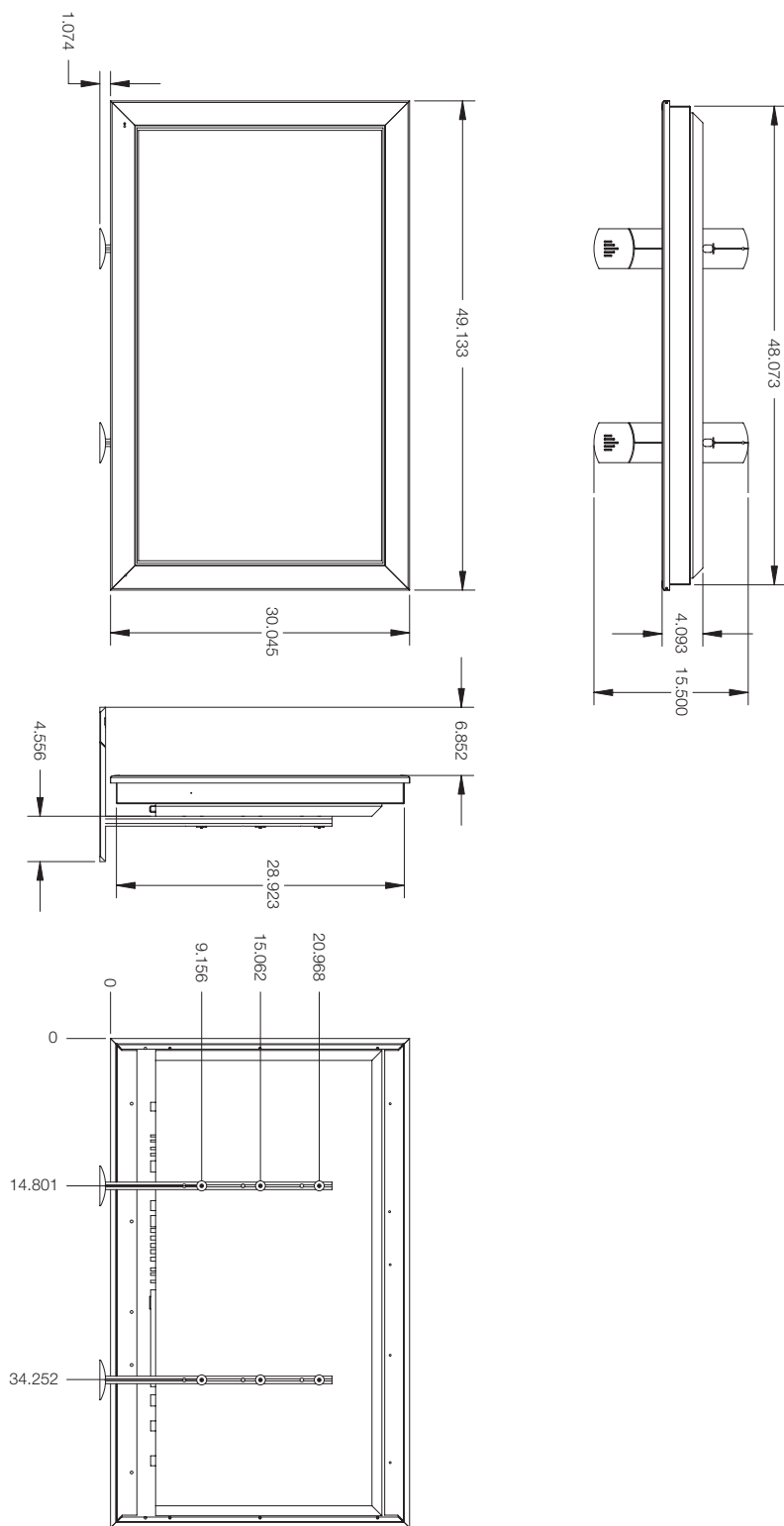
Figure 7-1. PlasmaWall Model PL-50XA Dimensions (with Optional Table Stand)
