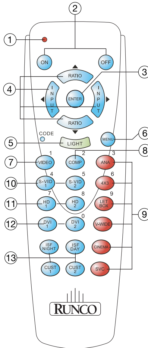
Figure 2-5. DHD Controller Remote Control
