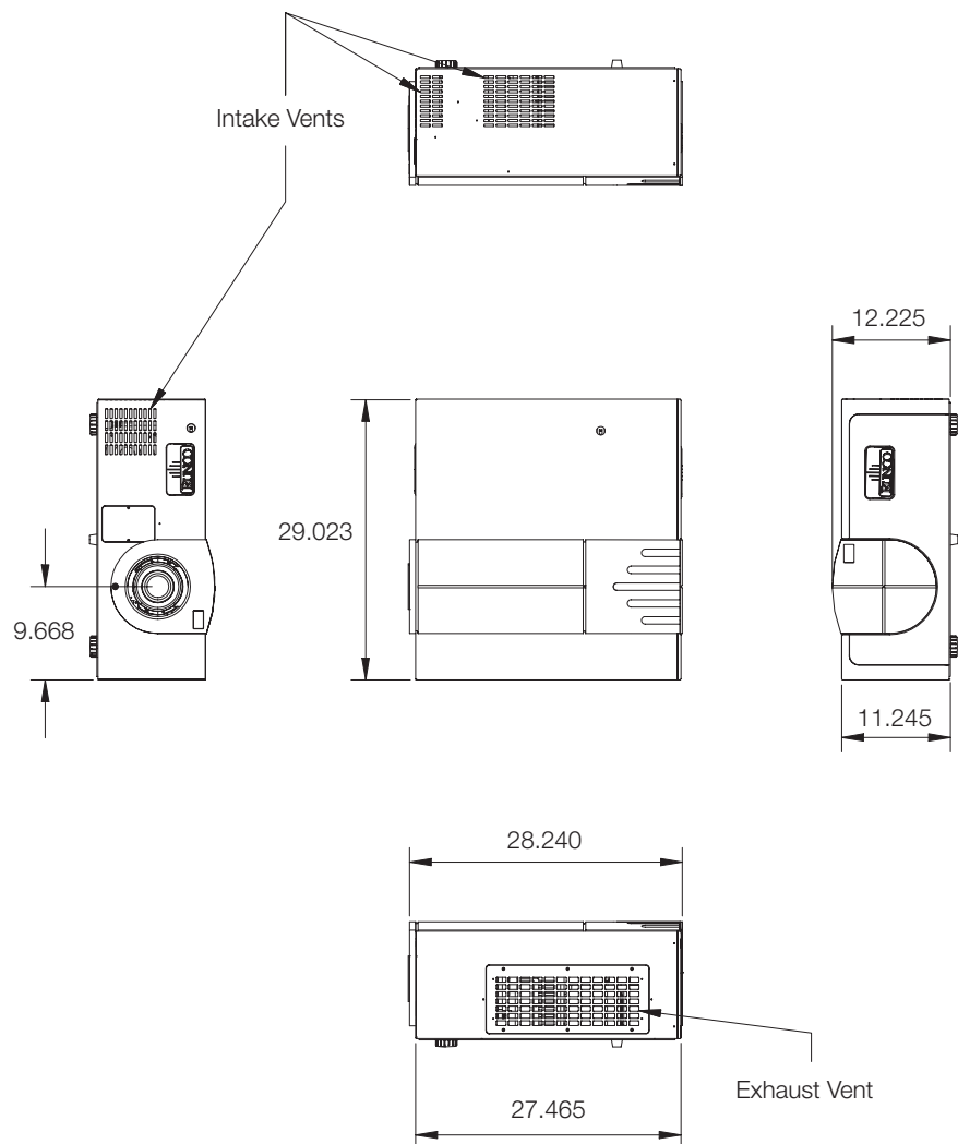
Figure 7-1. VX-40d/-50d/-60d/-80d Dimensions
