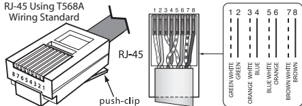
RJ-45 Using T568A Wiring Standard
