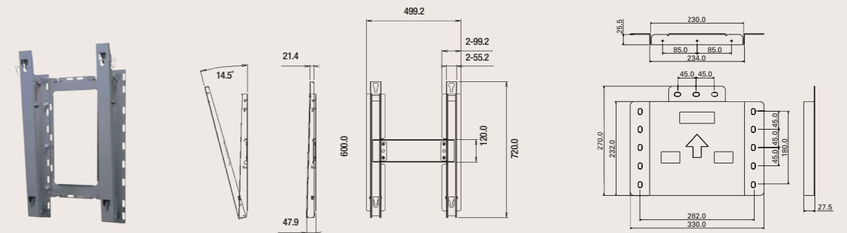
VMN4240D (400PX/400PXn/460PX/460PXn)
