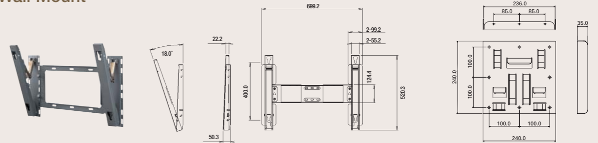
WMB-4050PS (400PX/400PXn/460PX/460PXn)
