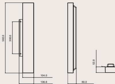
SP-L400PB/S (400PX/400PXn)
