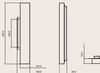
SP-L460PB/S (460PX/460PXn)
