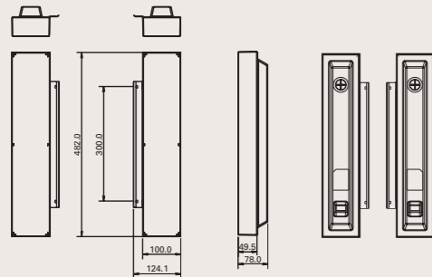
SP-L320PB/S (320PX)
