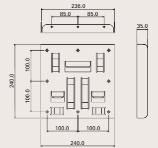
WML4001D (320PX)
