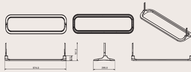
STN-323TB (400PX/400PXn/400TXn)
