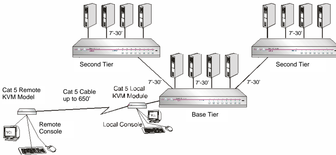
Figure 5 Two-Tier Configuration (with optional Remote Access)
