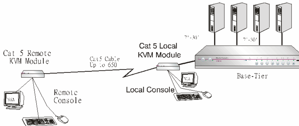
Figure 28 Remote Access with Cat5 Reach
