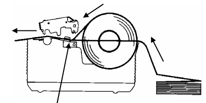
Route Paper under the Sensor
