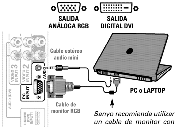
PANEL TRASERO HDTV
