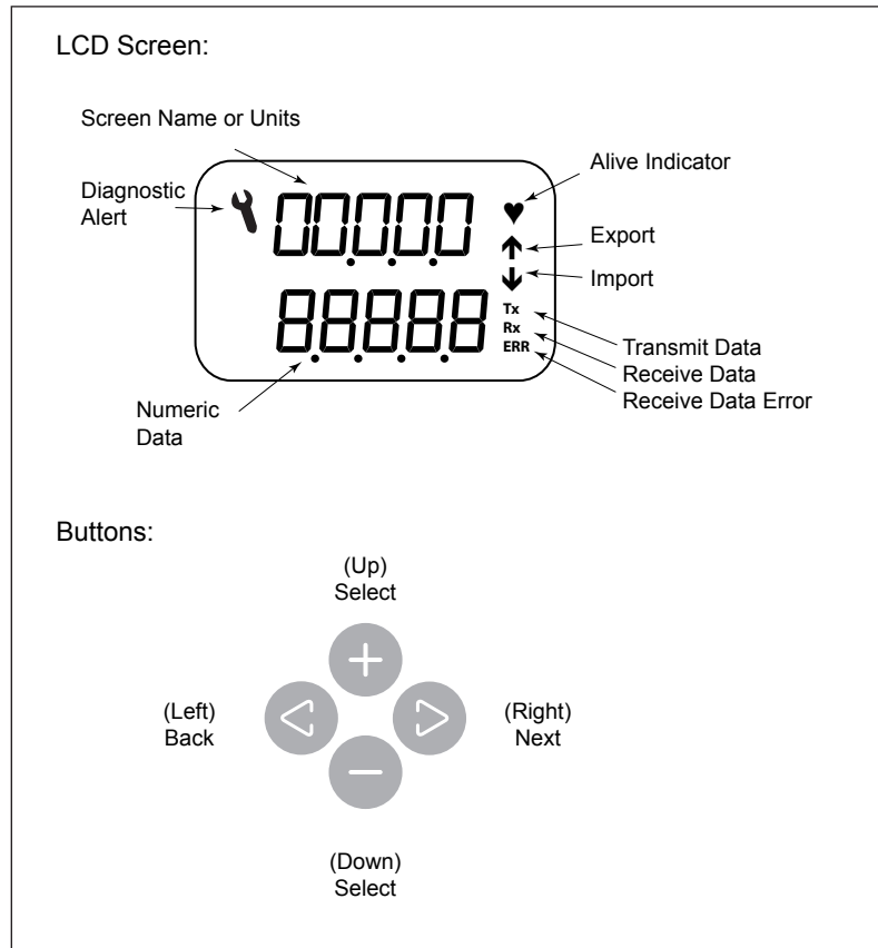
Figure 5 Display Screen
